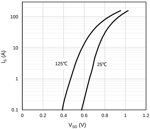
Figure 7: Body-Diode Characteristics
