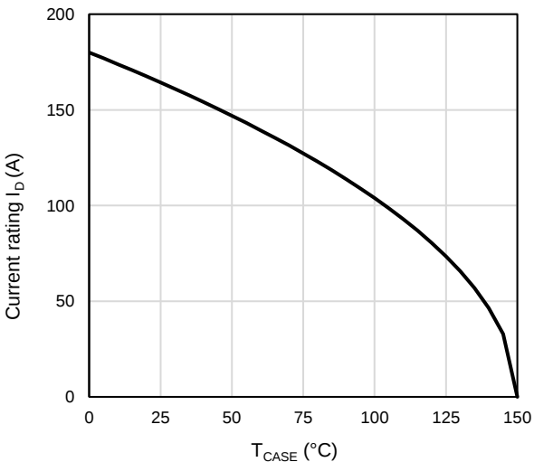
Figure 12: Current De-rating
