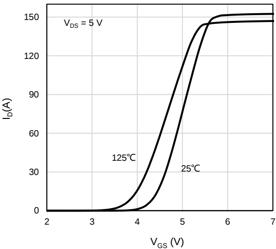
Figure 2: Transfer Characteristics
