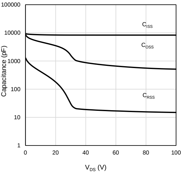
Figure 9: Capacitance Characteristics
